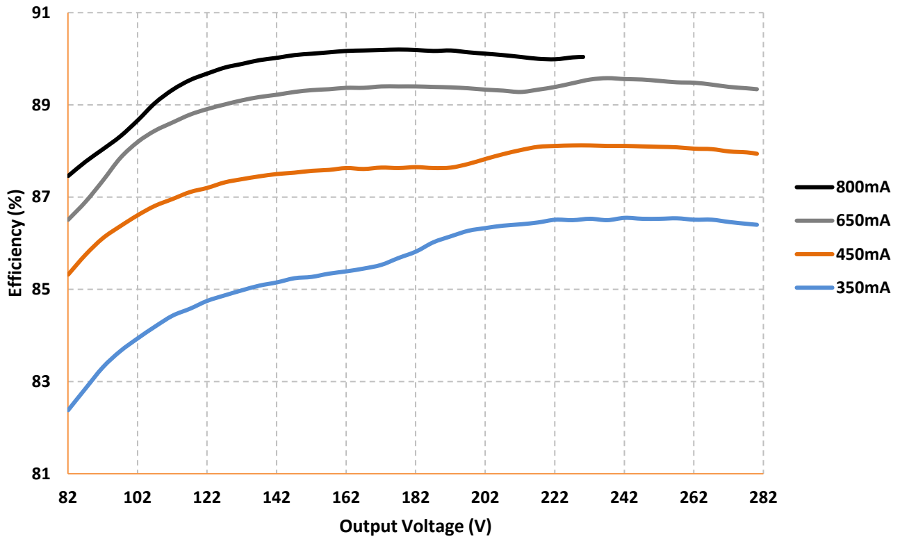
Efficiency @ 120V
