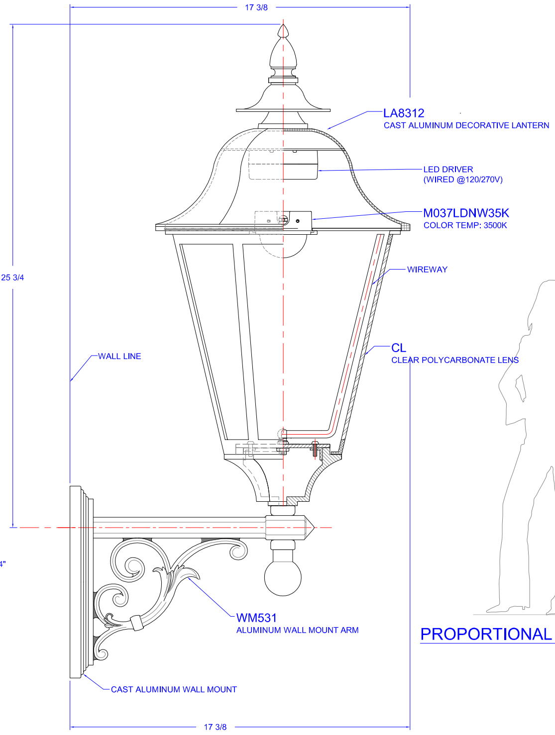
ELEVATION VIEW
