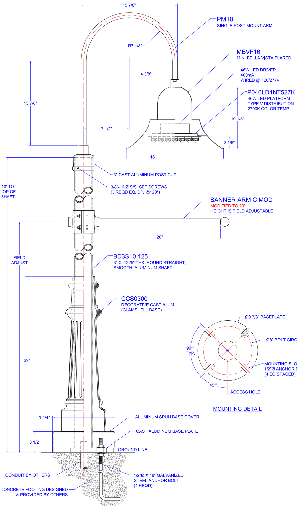
PROPORTIONAL VIEW
