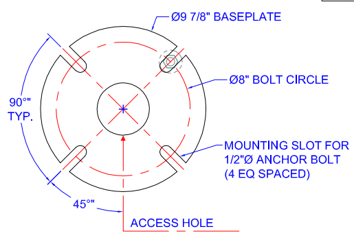
MOUNTING DETAIL
