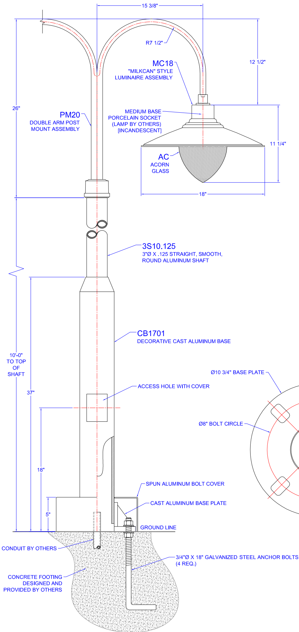
MOUNTING DETAIL
