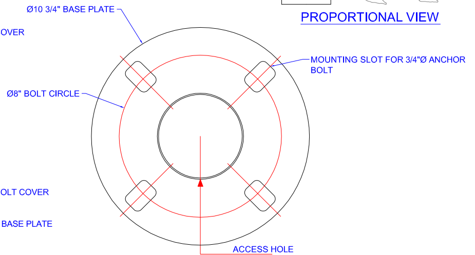
MOUNTING DETAIL
