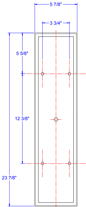
MOUNTING DETAIL
